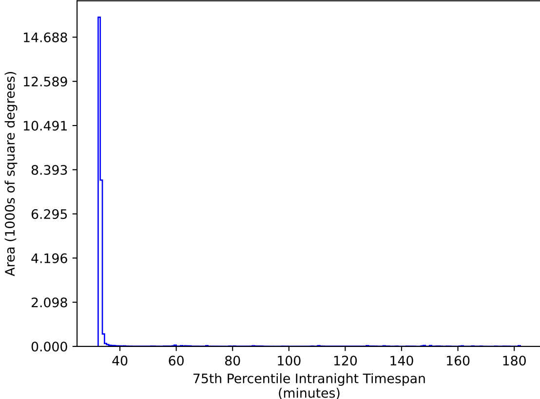
too_elab_r256_d3_ugrizy_v3.4_10yrs All sky y band: 75th Percentile Intranight Timespan
