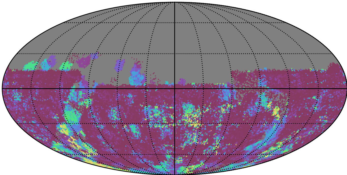
too_elab_r256_d3_ugrizy_v3.4_10yrs All sky u band: 75th Percentile Intranight Timespan
