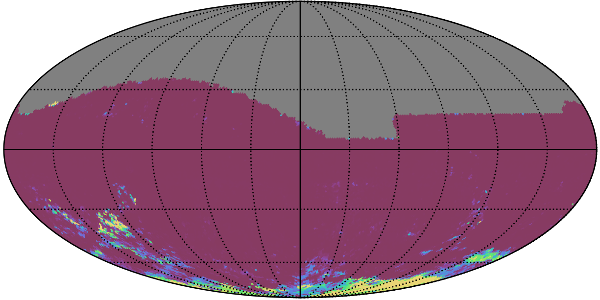
too_elab_r256_d3_ugrizy_v3.4_10yrs All sky ri bands: 75th Percentile Intranight Timespan
