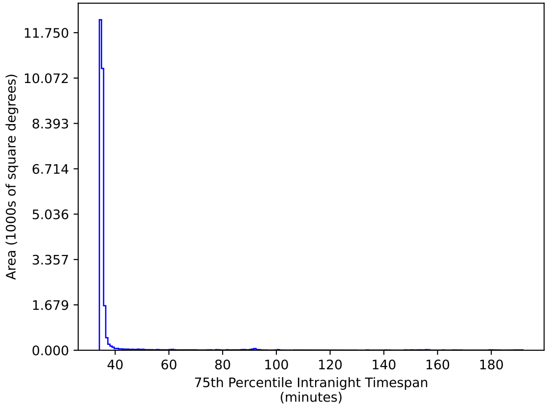
too_elab_r256_d3_ugrizy_v3.4_10yrs All sky ri bands: 75th Percentile Intranight Timespan
