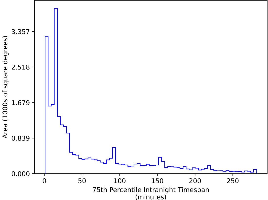
too_elab_r256_d3_ugrizy_v3.4_10yrs All sky r band: 75th Percentile Intranight Timespan
