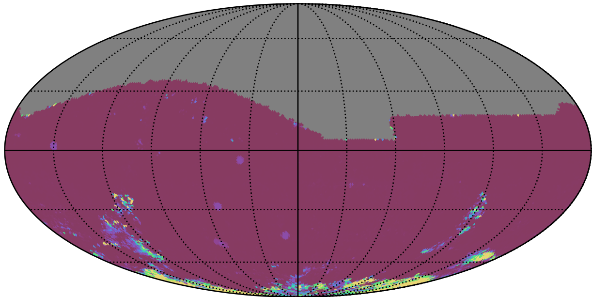
too_elab_r256_d3_ugrizy_v3.4_10yrs All sky iz bands: 75th Percentile Intranight Timespan
