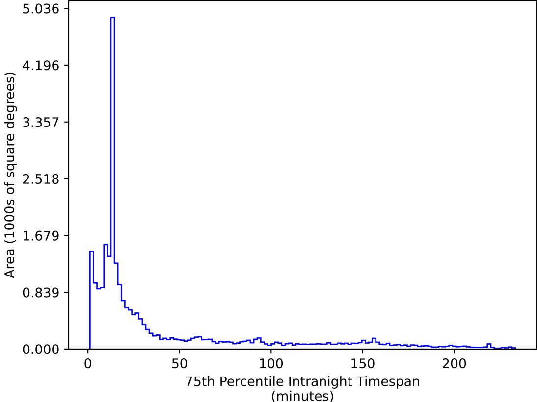
too_elab_r256_d3_ugrizy_v3.4_10yrs All sky i band: 75th Percentile Intranight Timespan
