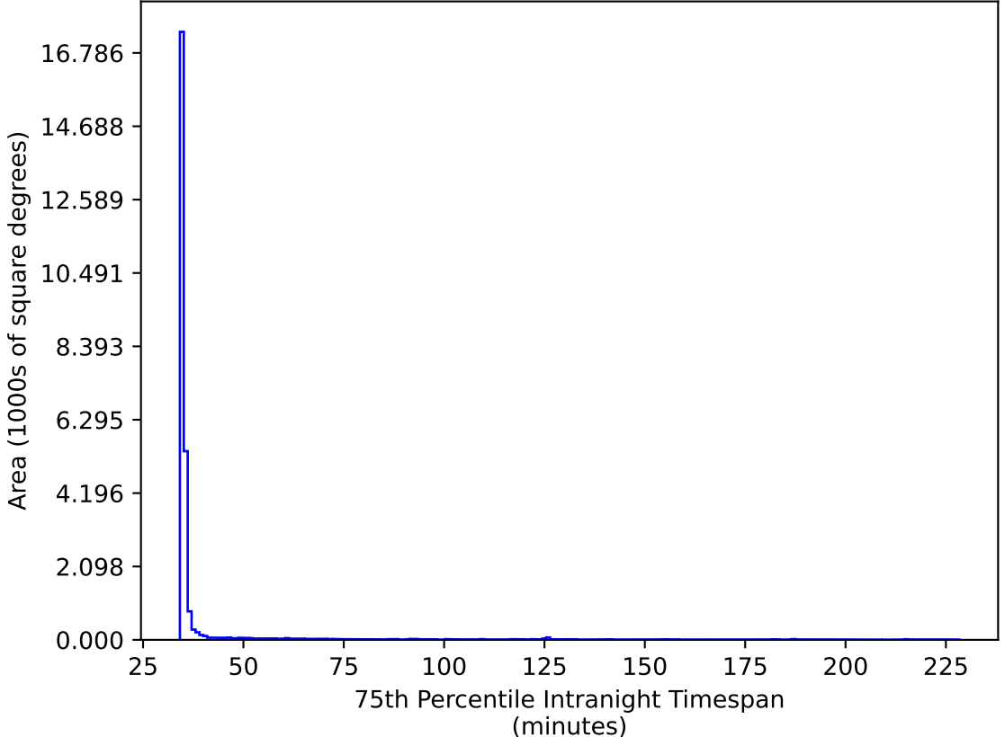
too_elab_r256_d3_ugrizy_v3.4_10yrs All sky gr bands: 75th Percentile Intranight Timespan
