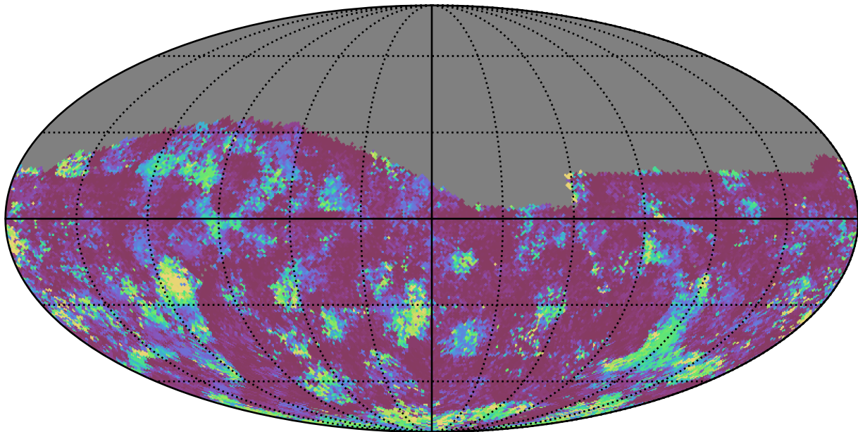
too_elab_r256_d3_ugrizy_v3.4_10yrs All sky g band: 75th Percentile Intranight Timespan
