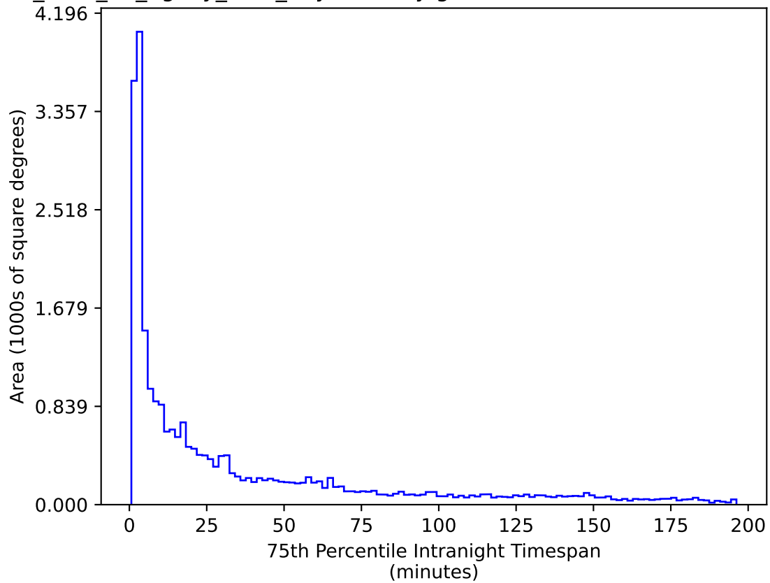
too_elab_r256_d3_ugrizy_v3.4_10yrs All sky g band: 75th Percentile Intranight Timespan
