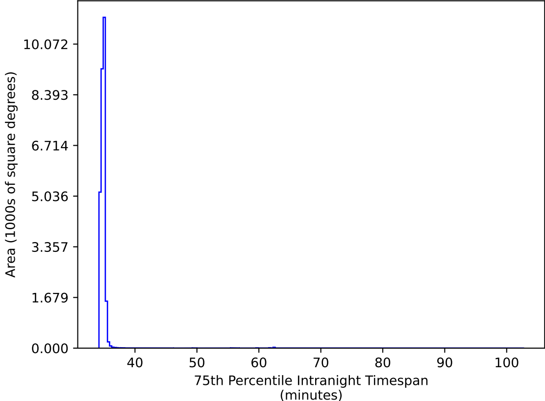
too_elab_r256_d3_ugrizy_v3.4_10yrs All sky all bands: 75th Percentile Intranight Timespan
