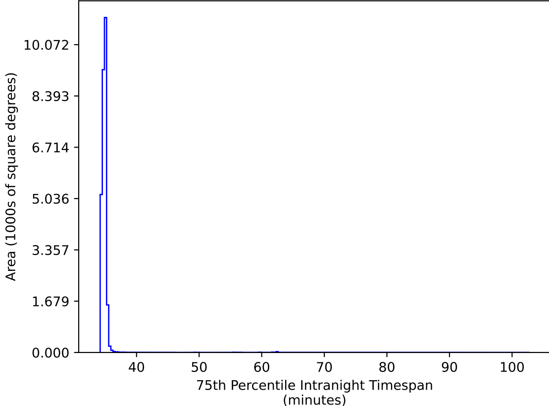
too_elab_r256_d3_ugrizy_v3.4_10yrs All sky: 75th Percentile Intranight Timespan
