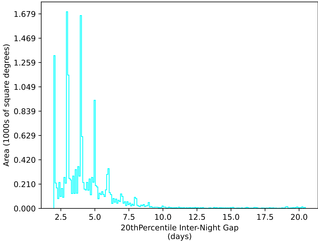
too_elab_r256_d3_ugrizy_v3.4_10yrs WFD u band: 20thPercentile Inter-Night Gap
