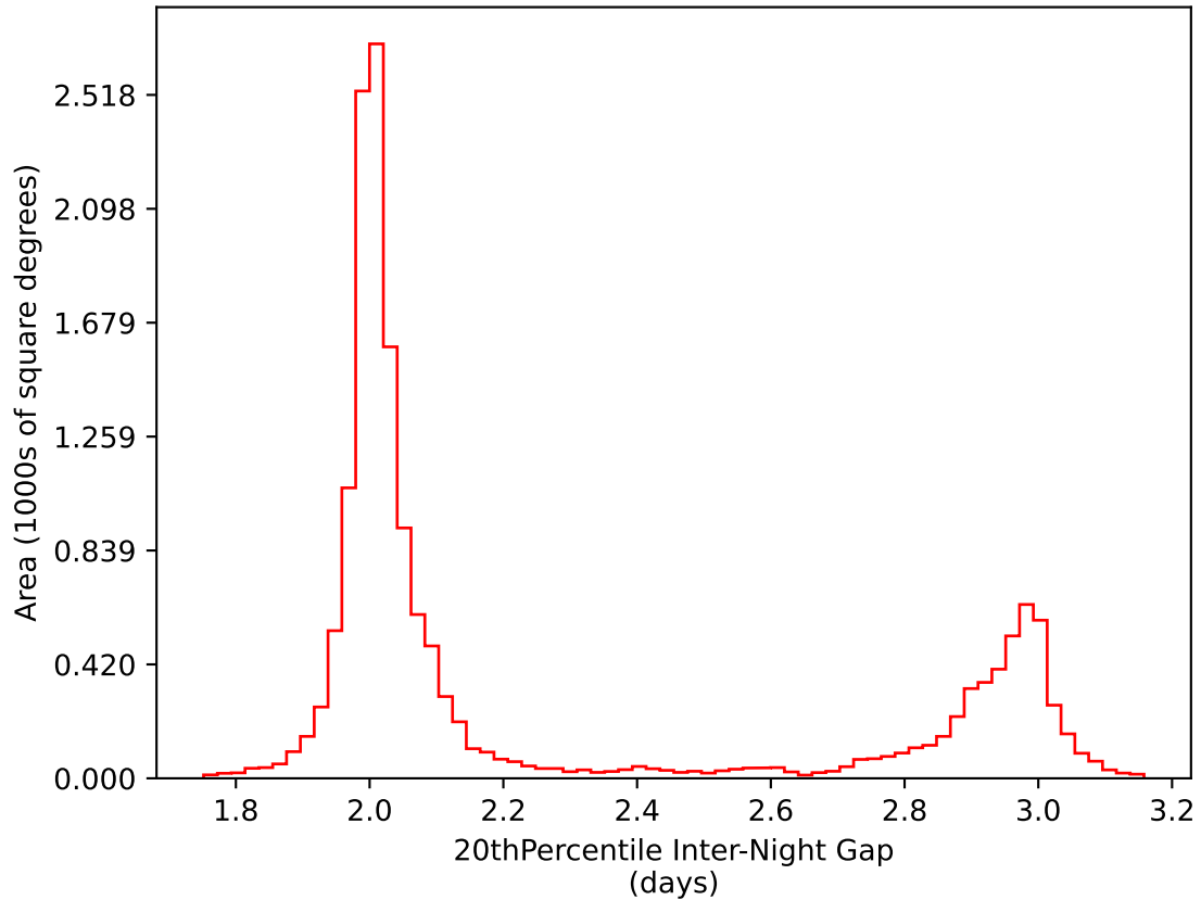
too_elab_r256_d3_ugrizy_v3.4_10yrs WFD i band: 20thPercentile Inter-Night Gap
