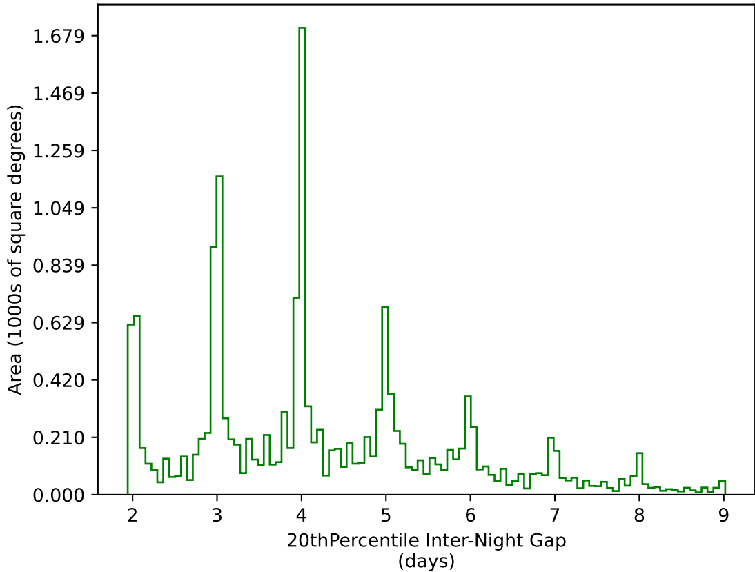
too_elab_r256_d3_ugrizy_v3.4_10yrs WFD g band: 20thPercentile Inter-Night Gap
