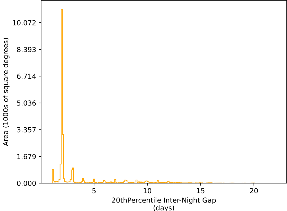
too_elab_r256_d3_ugrizy_v3.4_10yrs All sky r band: 20thPercentile Inter-Night Gap
