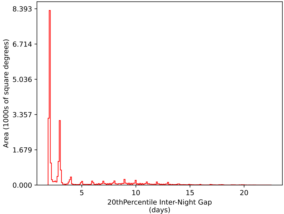
too_elab_r256_d3_ugrizy_v3.4_10yrs All sky i band: 20thPercentile Inter-Night Gap
