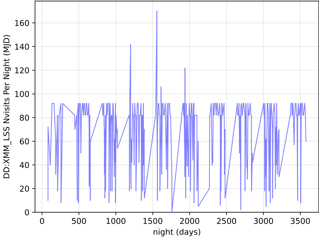
too_elab_r256_d3_ugrizy_v3.4_10yrs all bands: DD:XMM_LSS Nvisits Per Night
