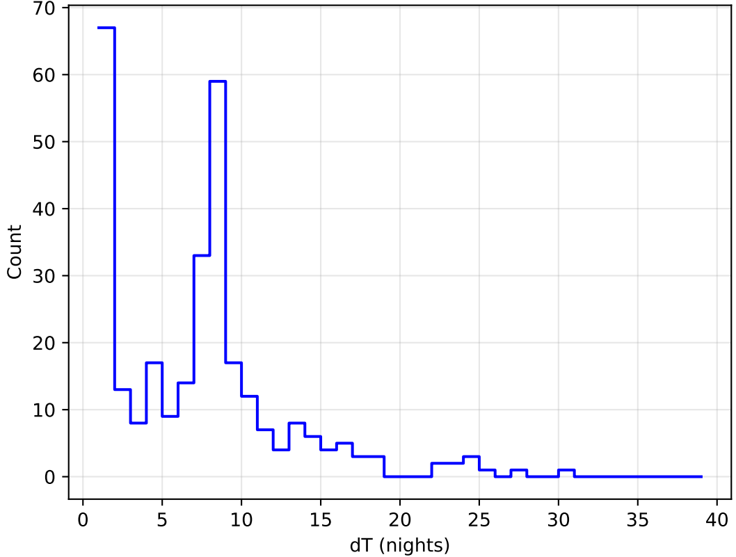
too_elab_r256_d3_ugrizy_v3.4_10yrs all bands: DD:XMM_LSS Delta Nights Histogram
