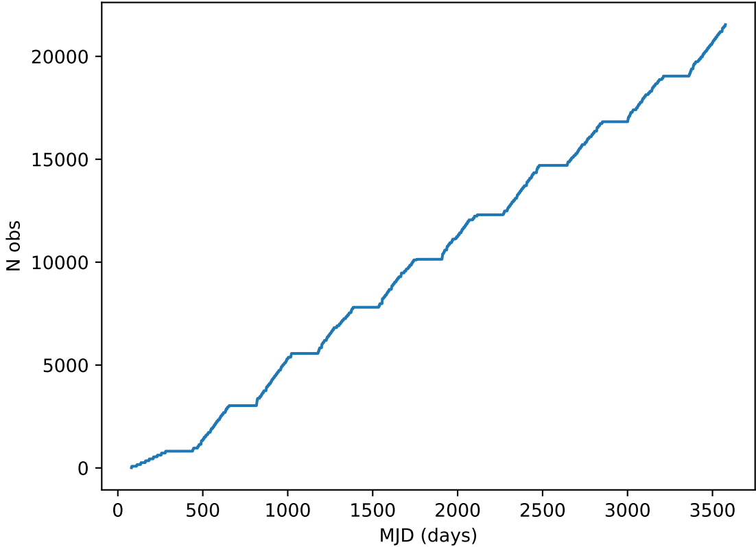
too_elab_r256_d3_ugrizy_v3.4_10yrs all bands: DD:XMM_LSS Cumulative NVisits
