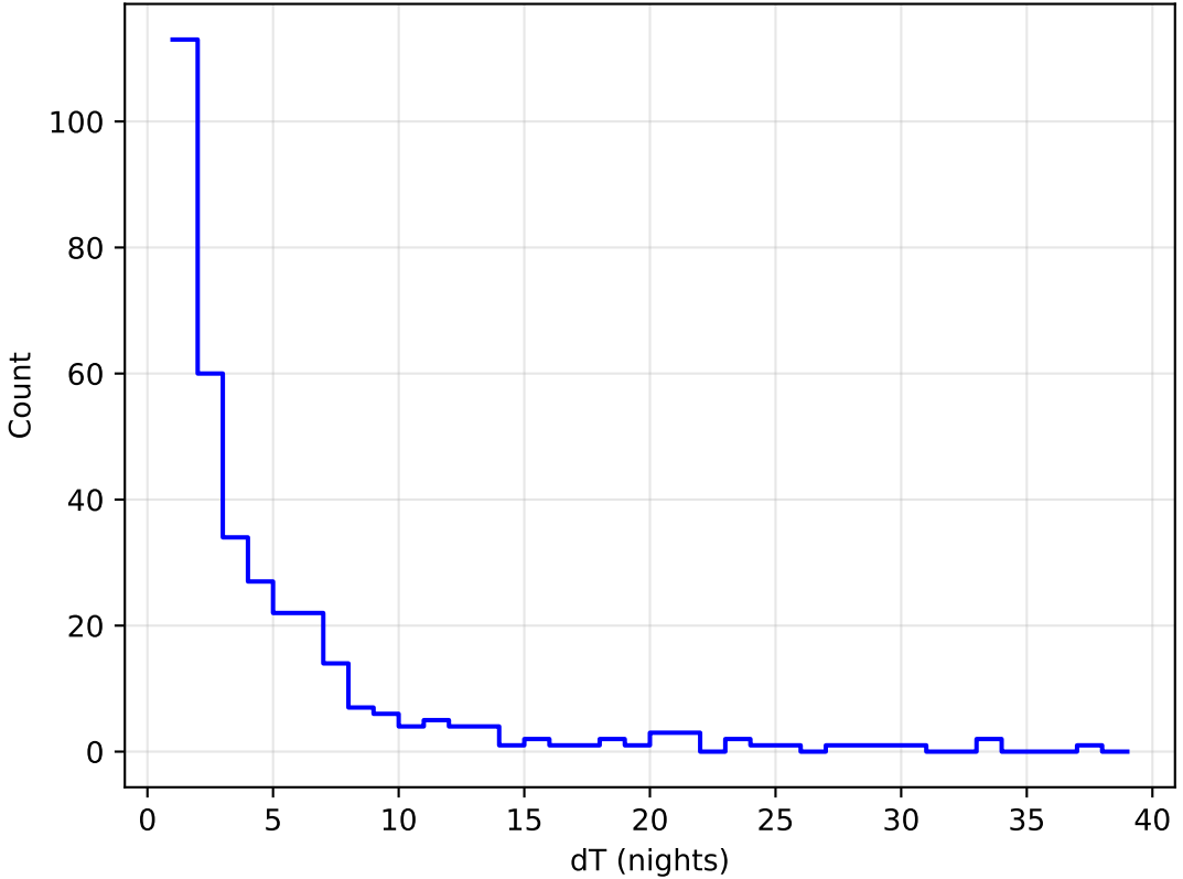
too_elab_r256_d3_ugrizy_v3.4_10yrs all bands: DD:WFD Delta Nights Histogram
