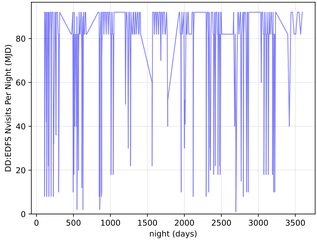
too_elab_r256_d3_ugrizy_v3.4_10yrs all bands: DD:EDFS Nvisits Per Night
