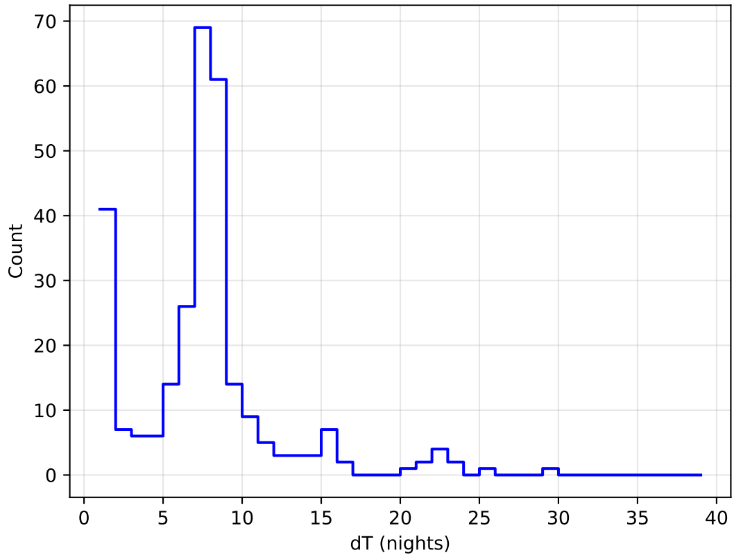
too_elab_r256_d3_ugrizy_v3.4_10yrs all bands: DD:ECDFS Delta Nights Histogram
