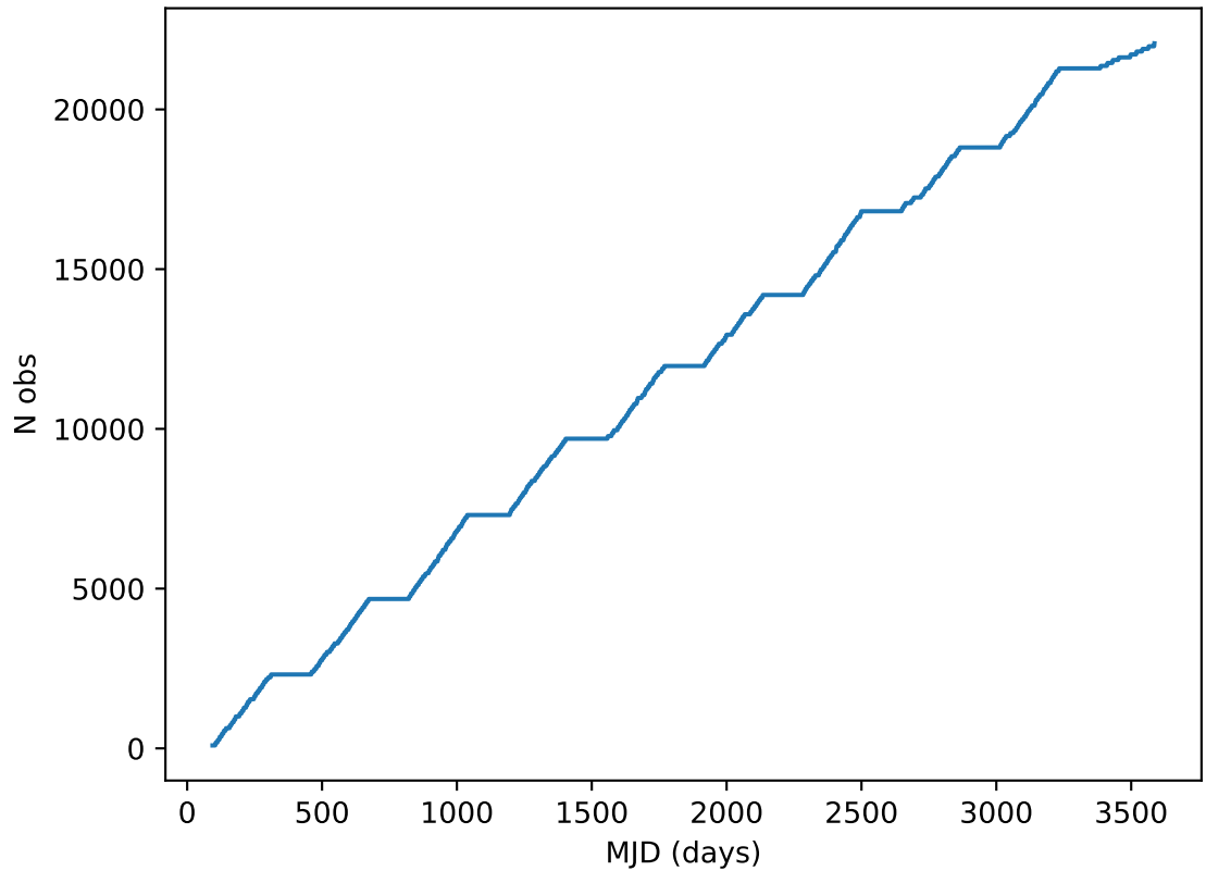
too_elab_r256_d3_ugrizy_v3.4_10yrs all bands: DD:ECDFS Cumulative NVisits
