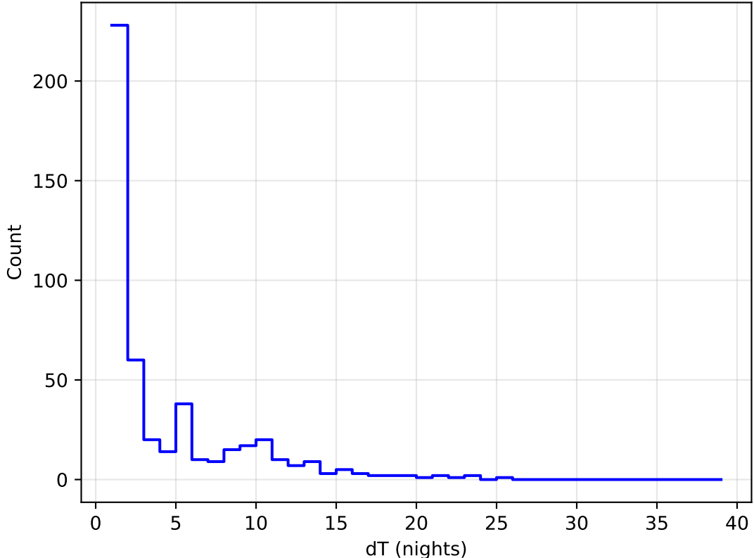
too_elab_r256_d3_ugrizy_v3.4_10yrs all bands: DD: COSMOS Delta Nights Histogram
