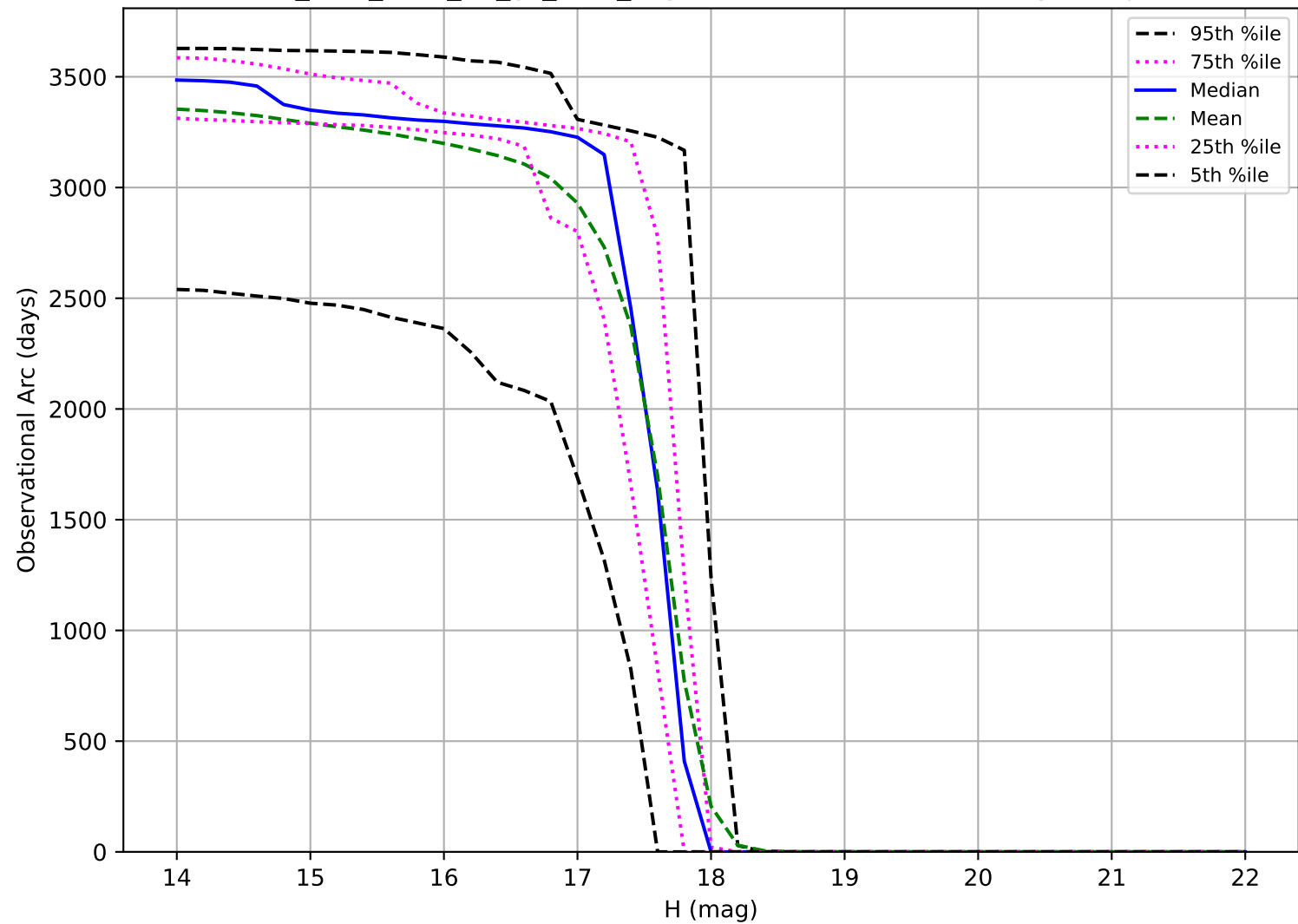
too_elab_r256_d3_gz_v3.4_10yrs: Observational Arc Length Trojan
