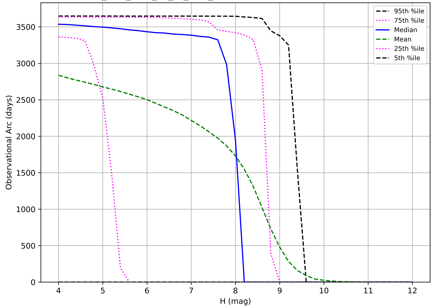
too_elab_r256_d3_gz_v3.4_10yrs: Observational Arc Length TNO
