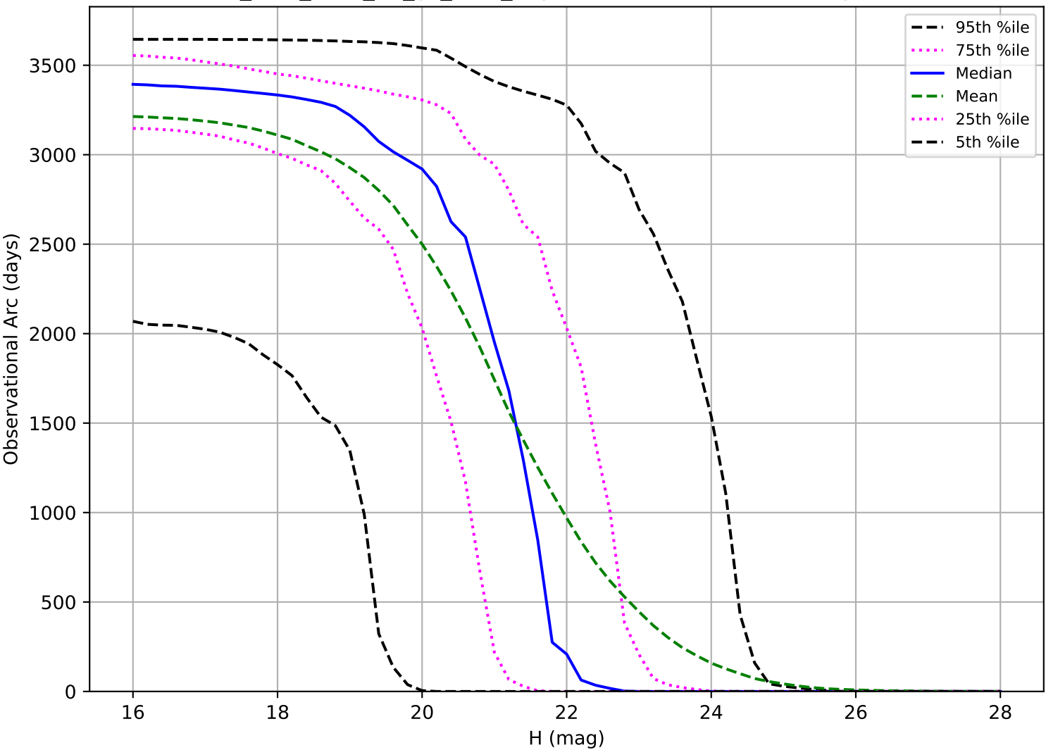
too_elab_r256_d3_gz_v3.4_10yrs: Observational Arc Length PHA
