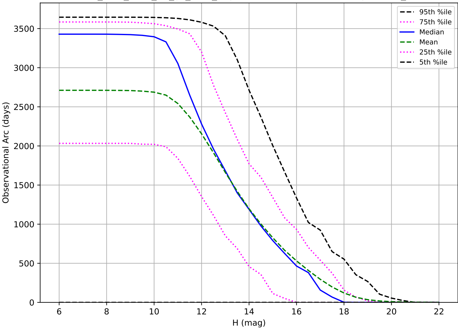
too_elab_r256_d3_gz_v3.4_10yrs: Observational Arc Length OCC_r5
