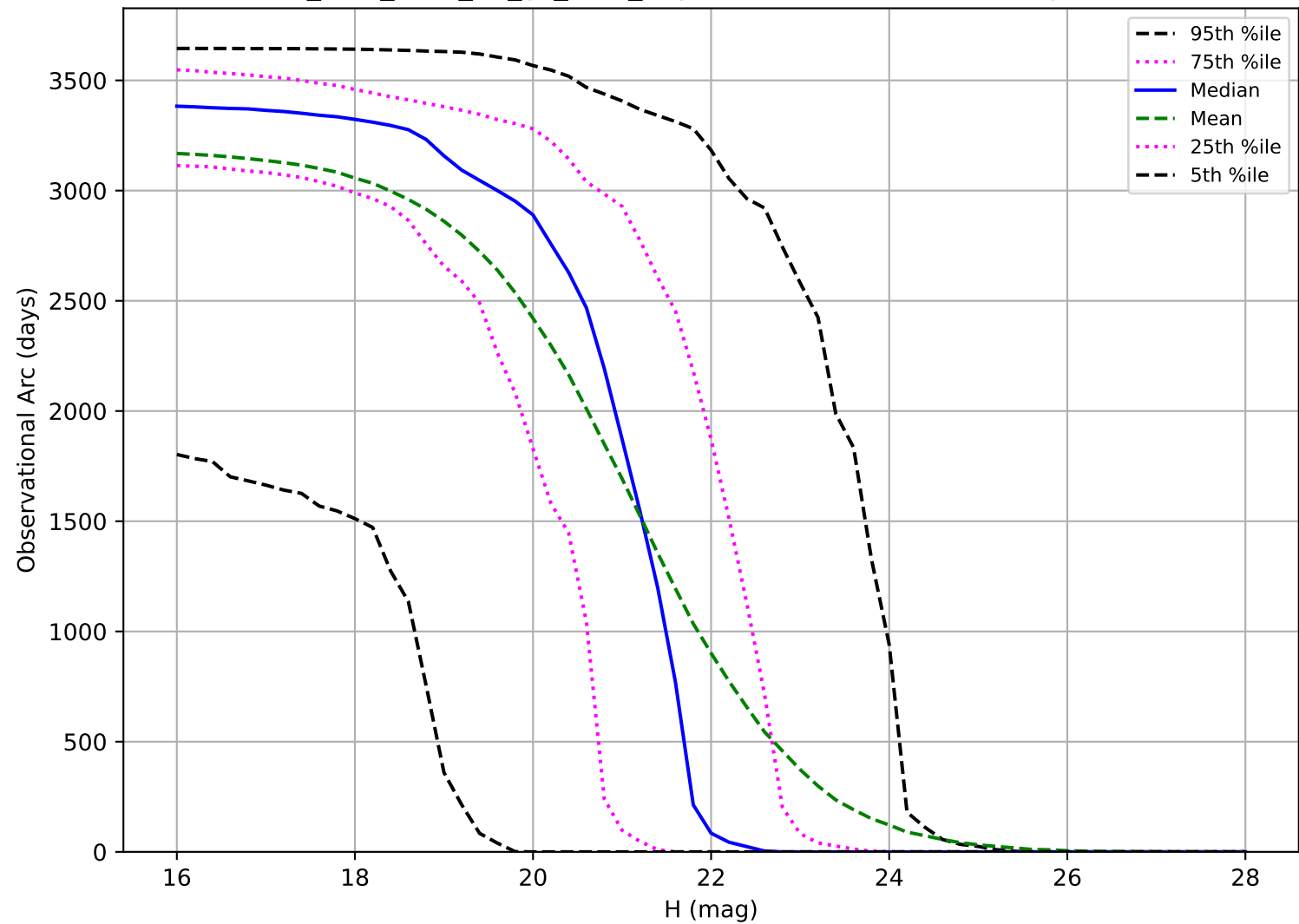
too_elab_r256_d3_gz_v3.4_10yrs: Observational Arc Length NEO
