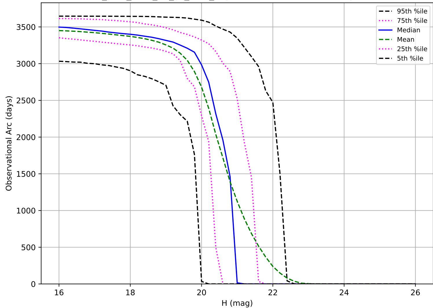
too_elab_r256_d3_gz_v3.4_10yrs: Observational Arc Length MBA
