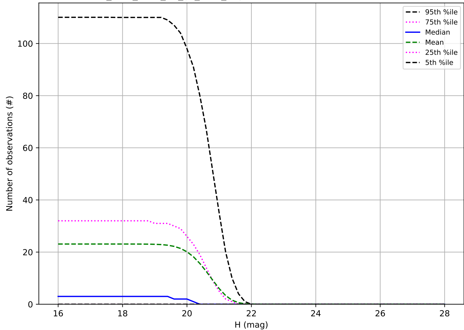
too_elab_r256_d3_gz_v3.4_10yrs: Number of observations Vatira
