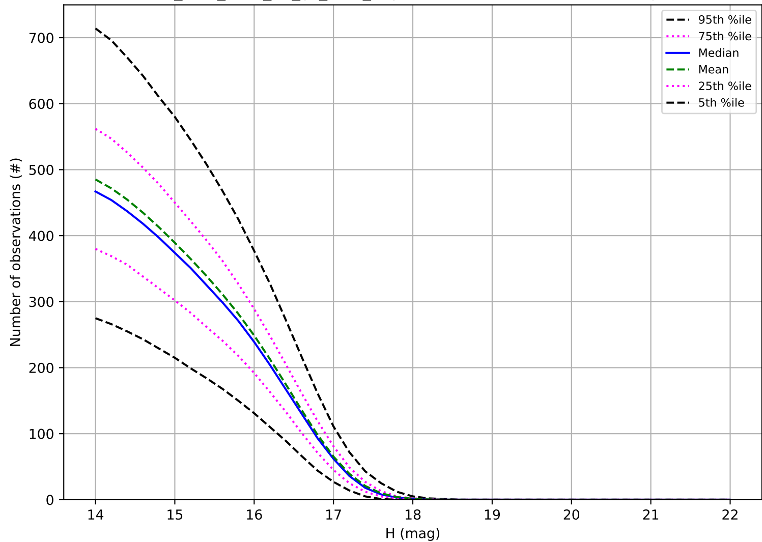
too_elab_r256_d3_gz_v3.4_10yrs: Number of observations Trojan
