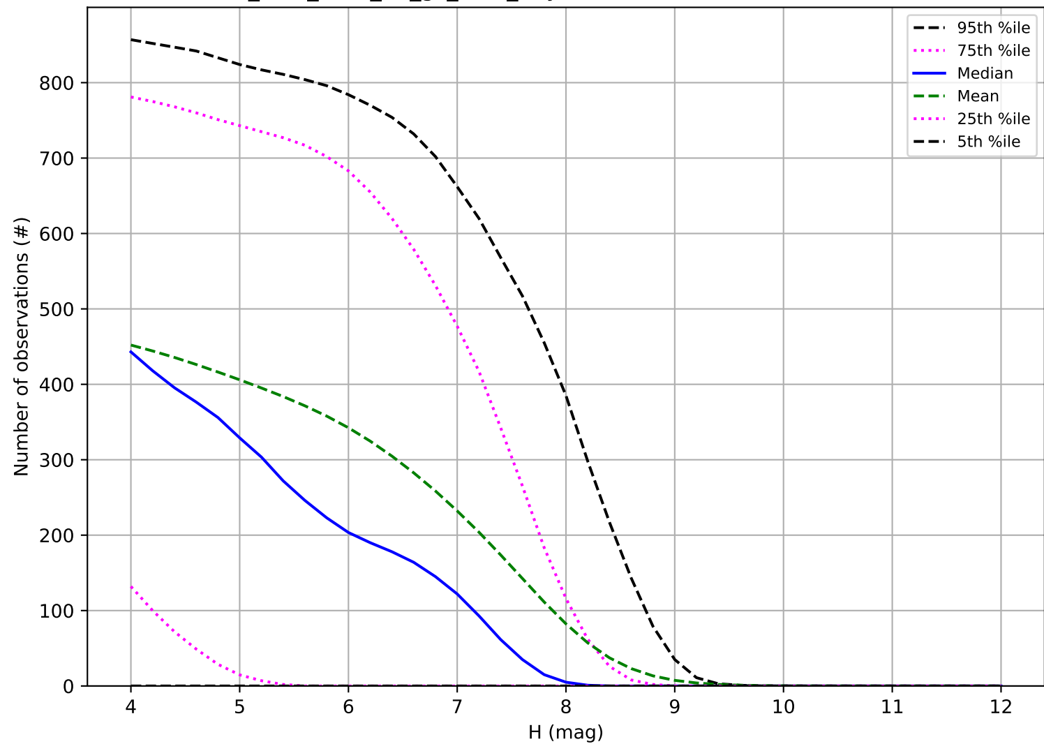
too_elab_r256_d3_gz_v3.4_10yrs: Number of observations TNO
