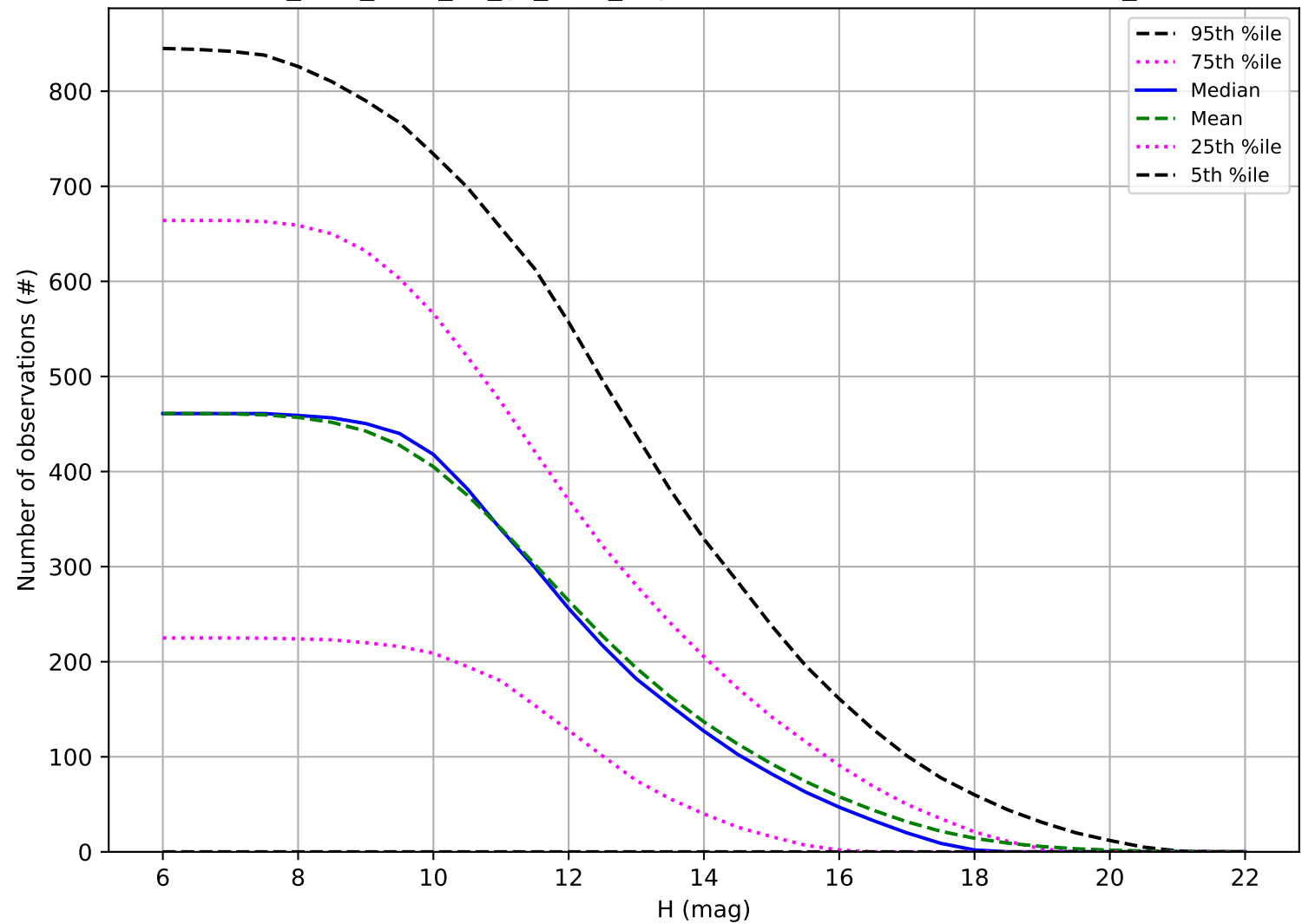
too_elab_r256_d3_gz_v3.4_10yrs: Number of observations OCC_r5
