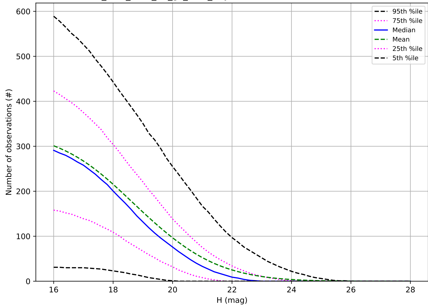
too_elab_r256_d3_gz_v3.4_10yrs: Number of observations NEO
