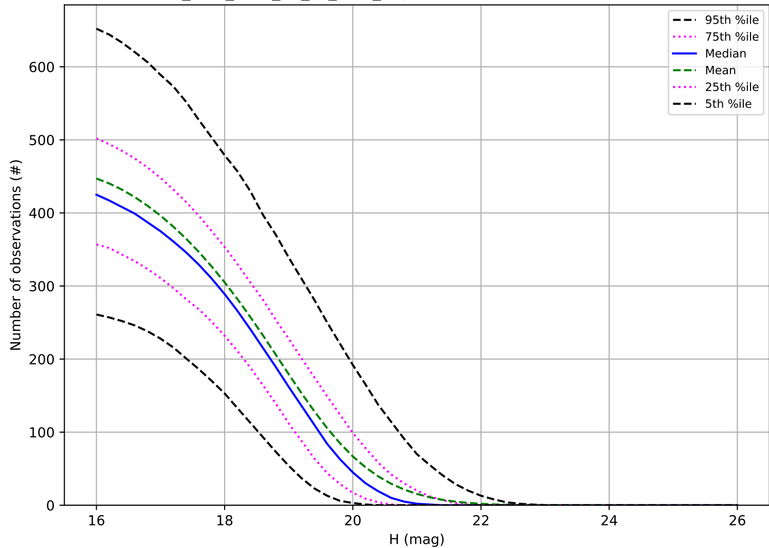
too_elab_r256_d3_gz_v3.4_10yrs: Number of observations MBA
