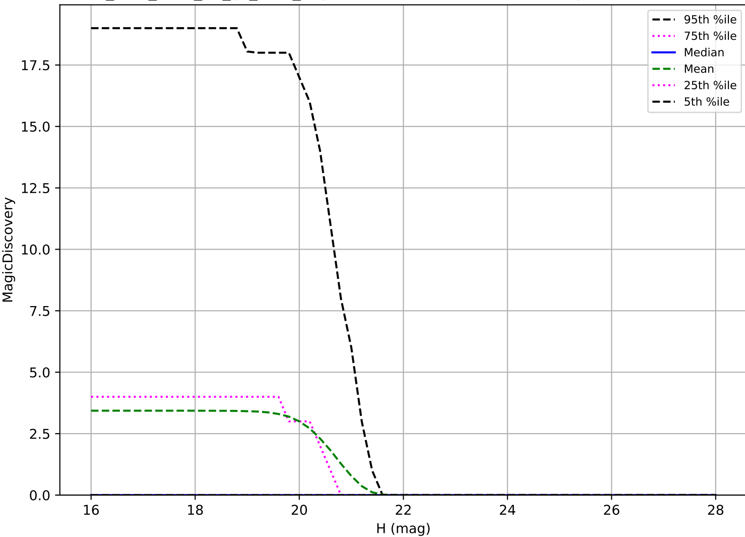
too_elab_r256_d3_gz_v3.4_10yrs: Vatira 6 detections in 60 nights detection loss
