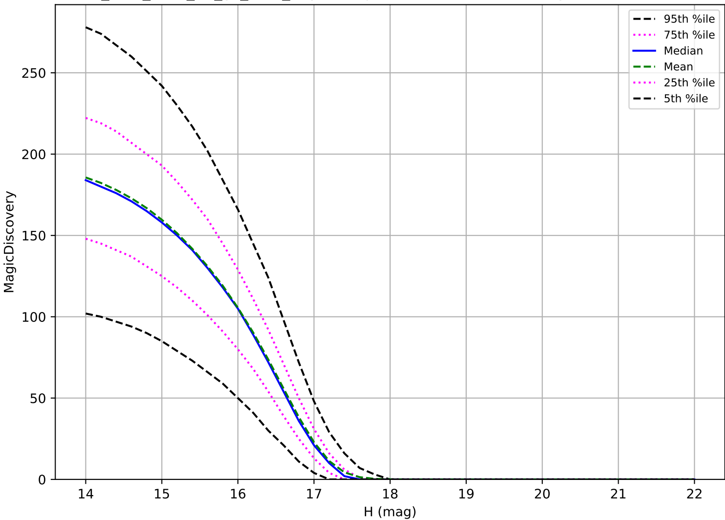
too_elab_r256_d3_gz_v3.4_10yrs: Trojan 6 detections in 60 nights detection loss
