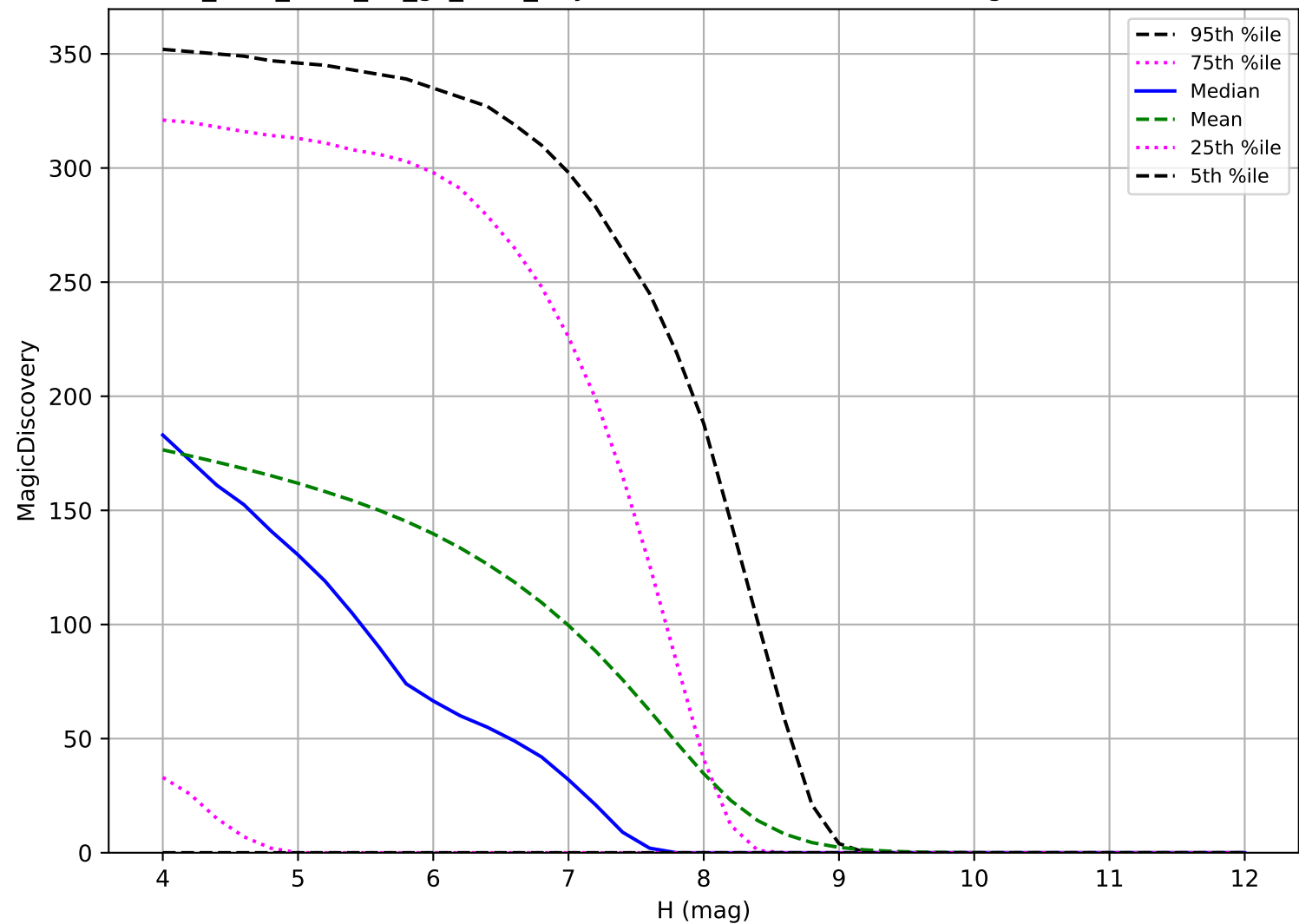
too_elab_r256_d3_gz_v3.4_10yrs: TNO 6 detections in 60 nights detection loss
