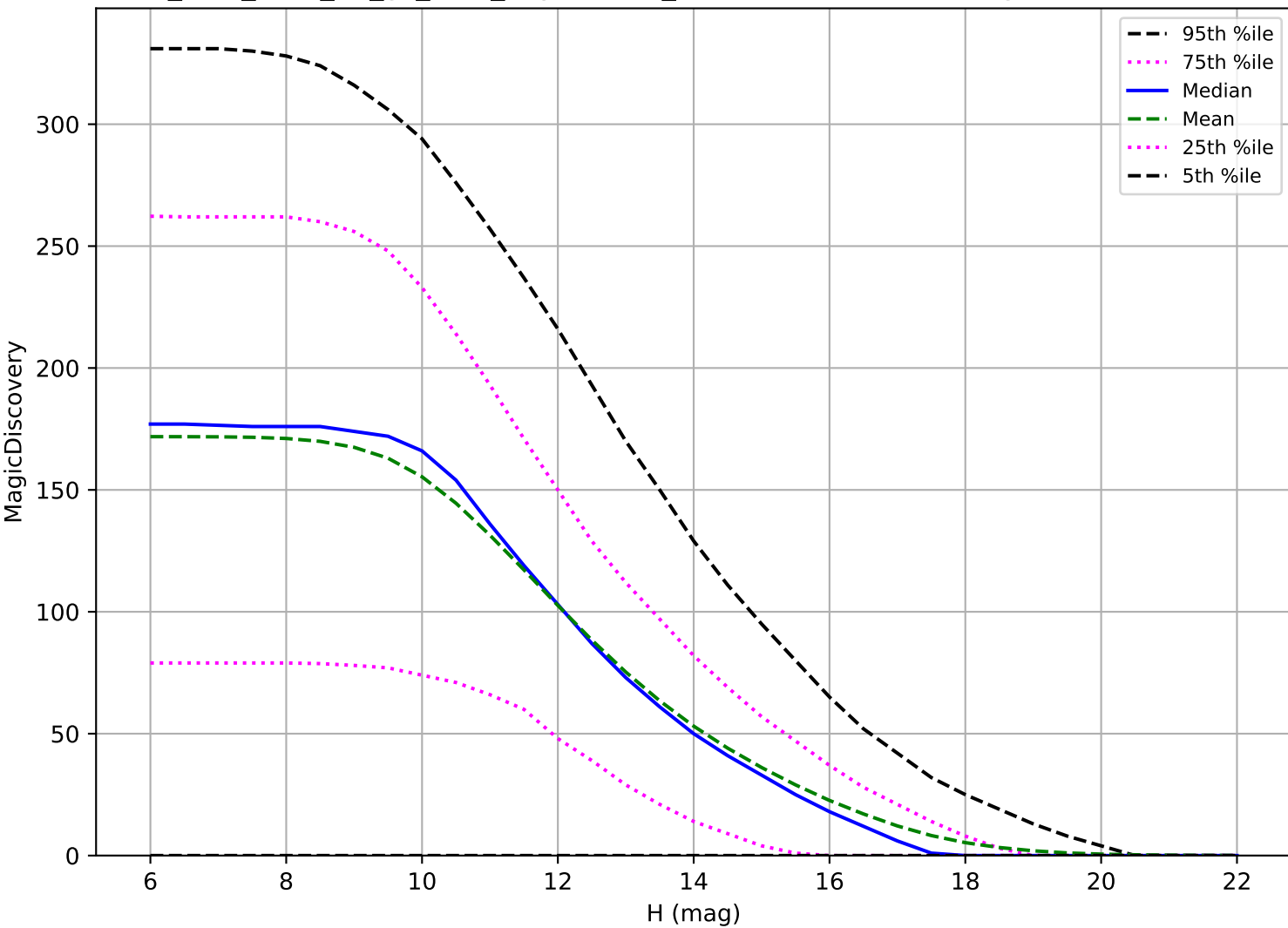
too_elab_r256_d3_gz_v3.4_10yrs: OCC_r5 6 detections in 60 nights detection loss
