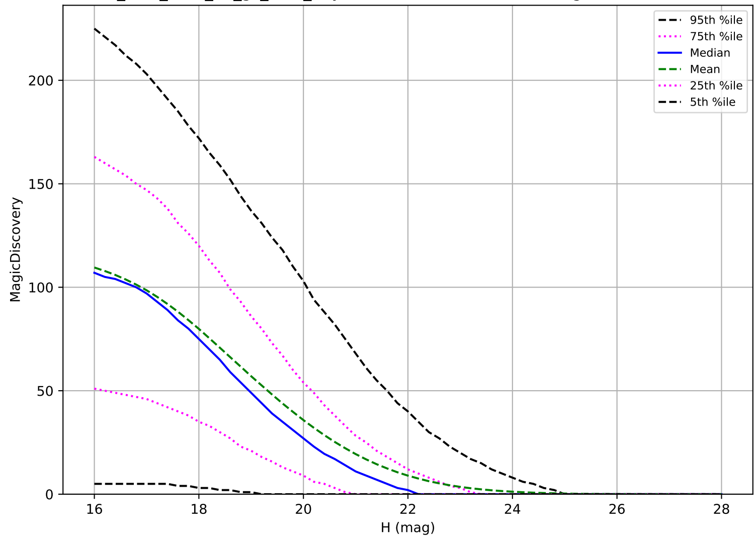
too_elab_r256_d3_gz_v3.4_10yrs: NEO 6 detections in 60 nights detection loss
