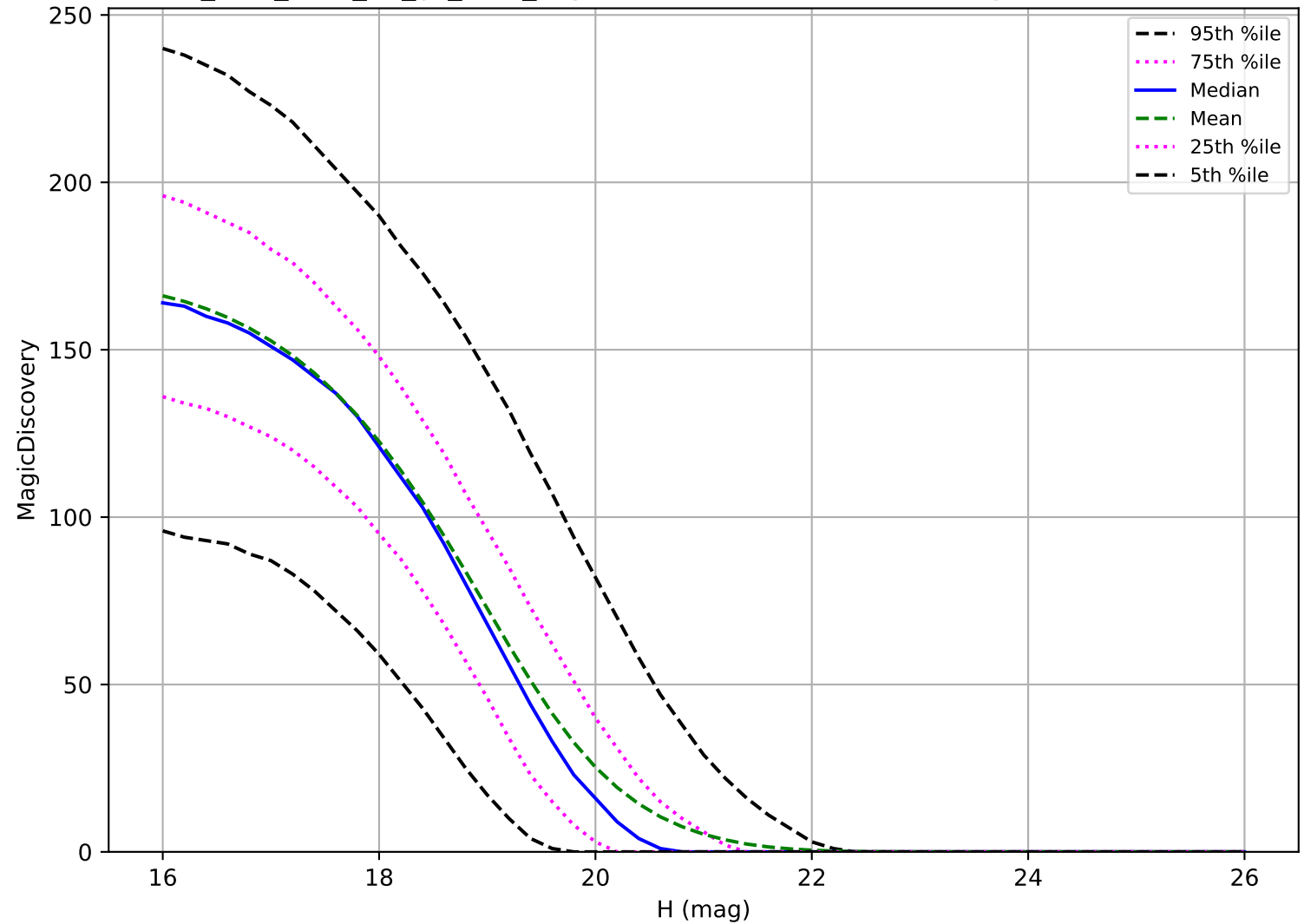
too_elab_r256_d3_gz_v3.4_10yrs: MBA 6 detections in 60 nights detection loss
