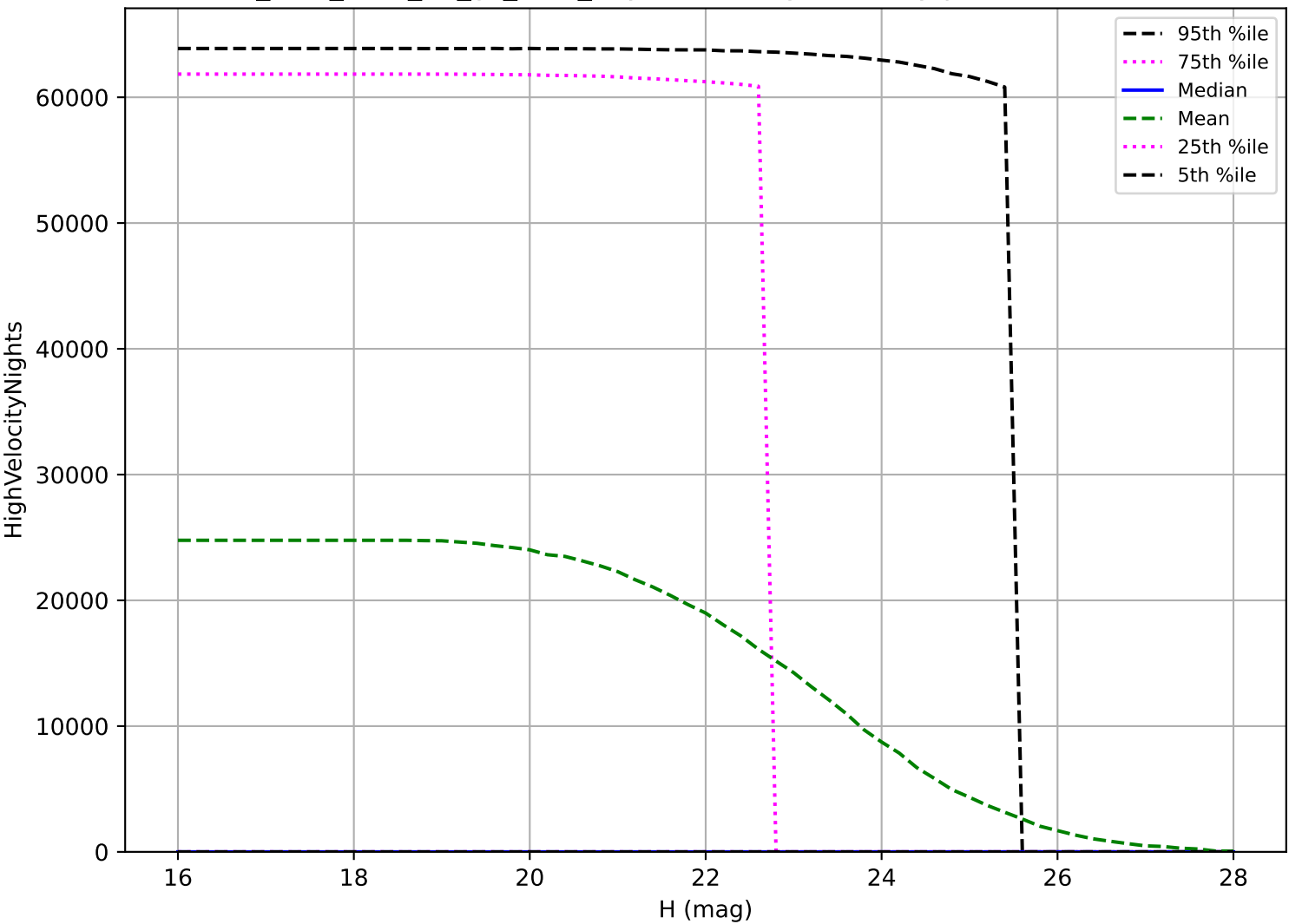
too_elab_r256_d3_gz_v3.4_10yrs: PHA High velocity pair detection loss
