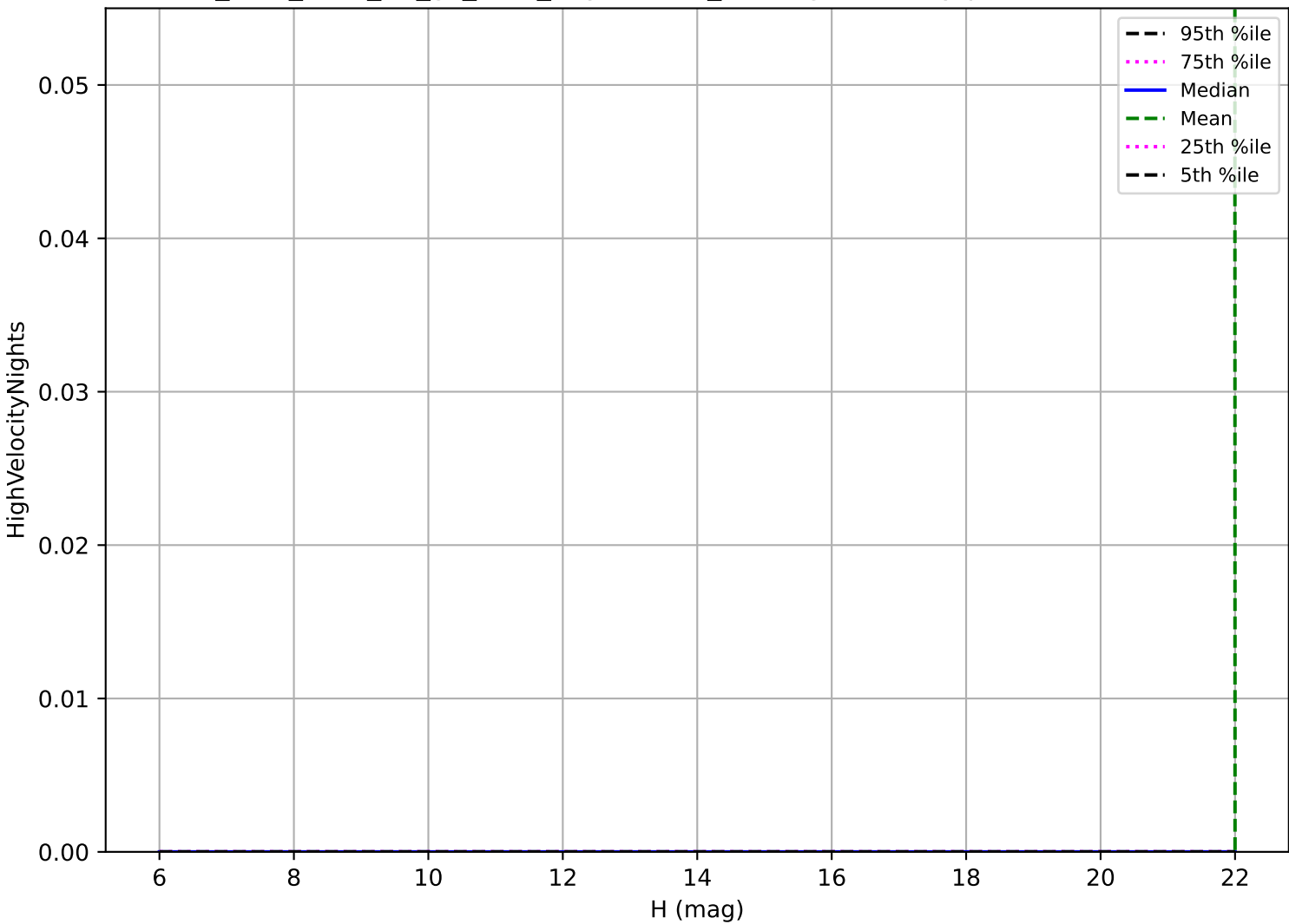
too_elab_r256_d3_gz_v3.4_10yrs: OCC_r20 High velocity pair detection loss
