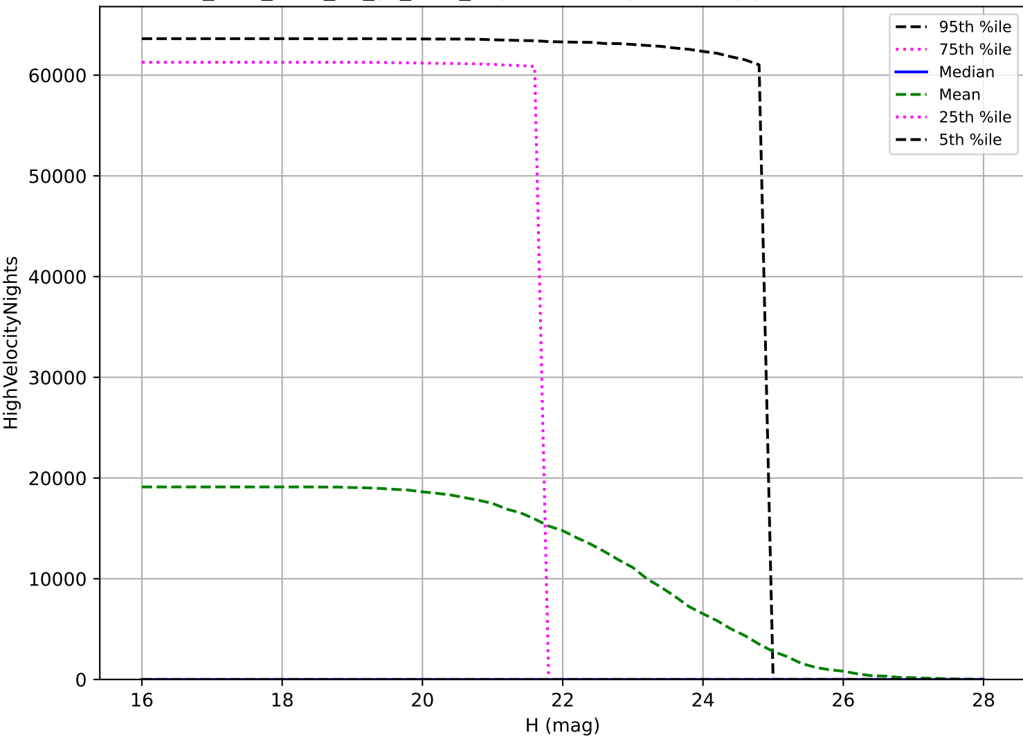
too_elab_r256_d3_gz_v3.4_10yrs: NEO High velocity pair detection loss
