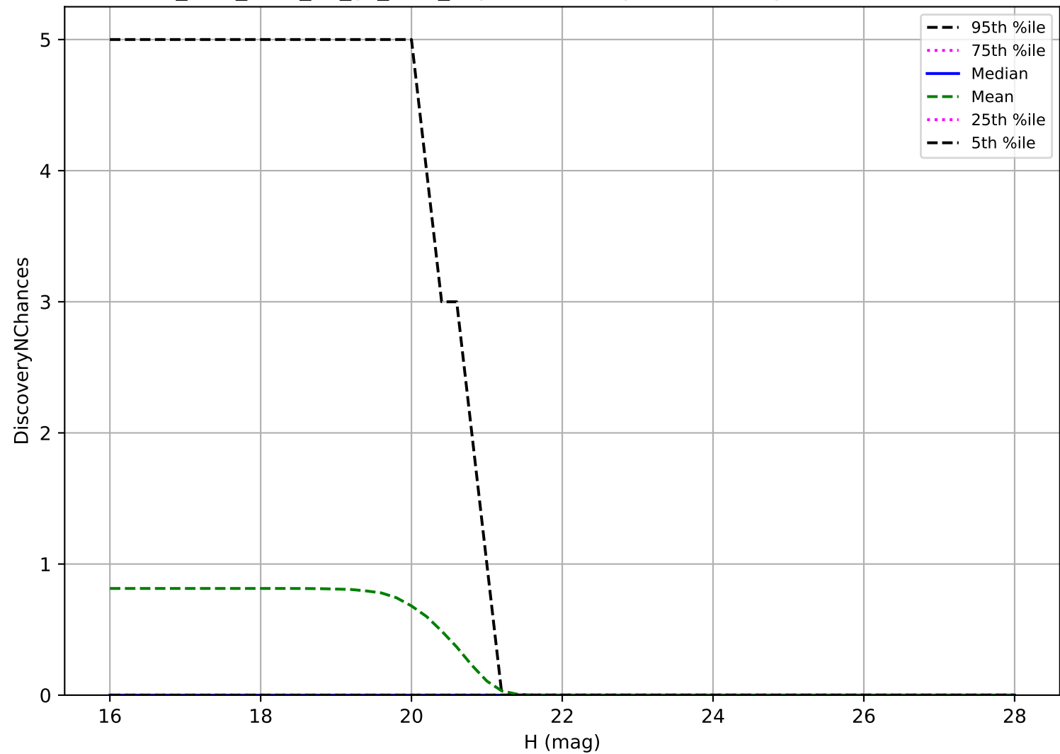
too_elab_r256_d3_gz_v3.4_10yrs: Vatira 3 pairs in 15 nights detection loss
