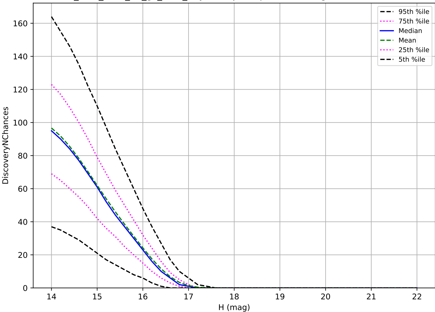
too_elab_r256_d3_gz_v3.4_10yrs: Trojan 3 pairs in 15 nights detection loss
