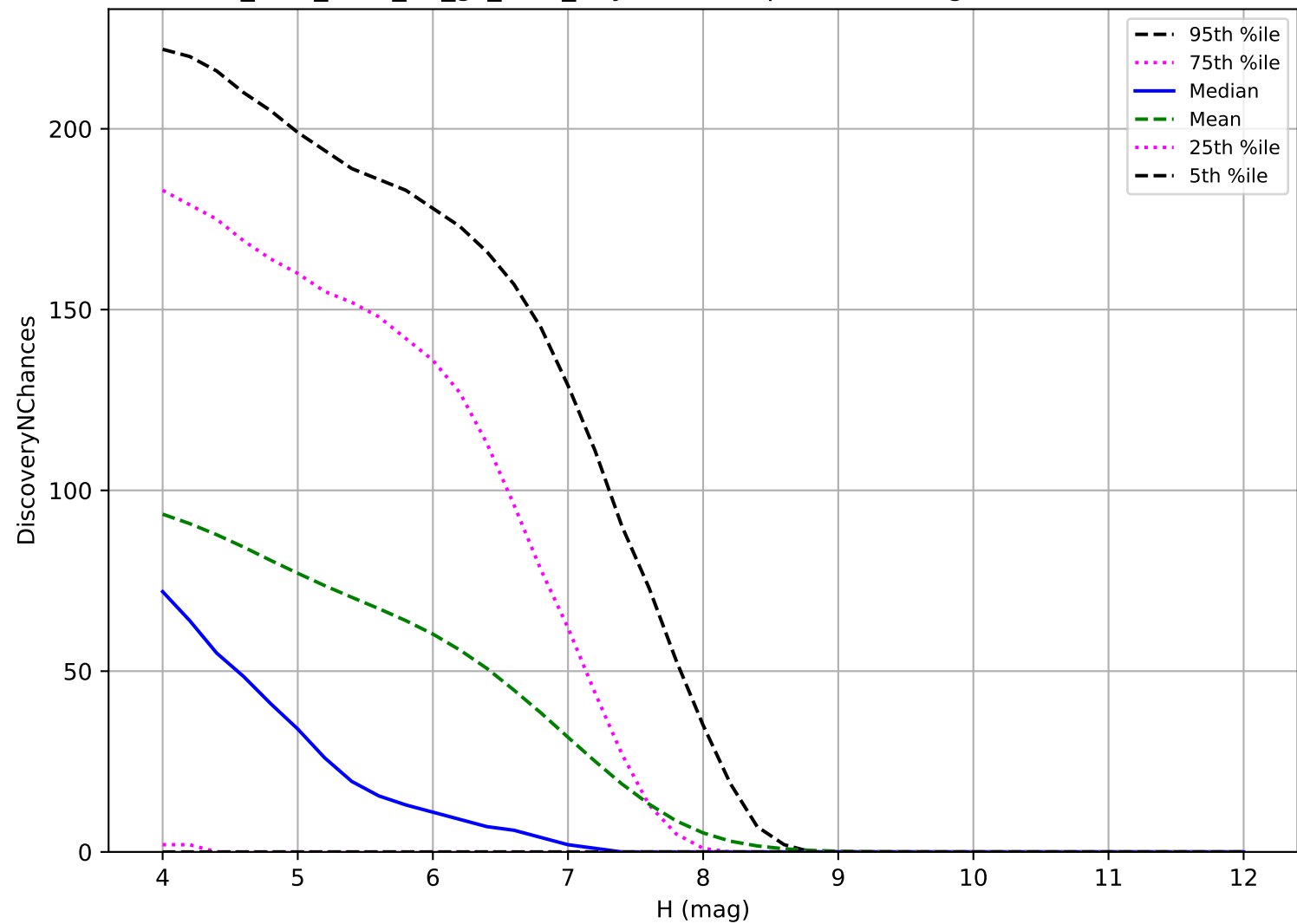
too_elab_r256_d3_gz_v3.4_10yrs: TNO 3 pairs in 15 nights detection loss
