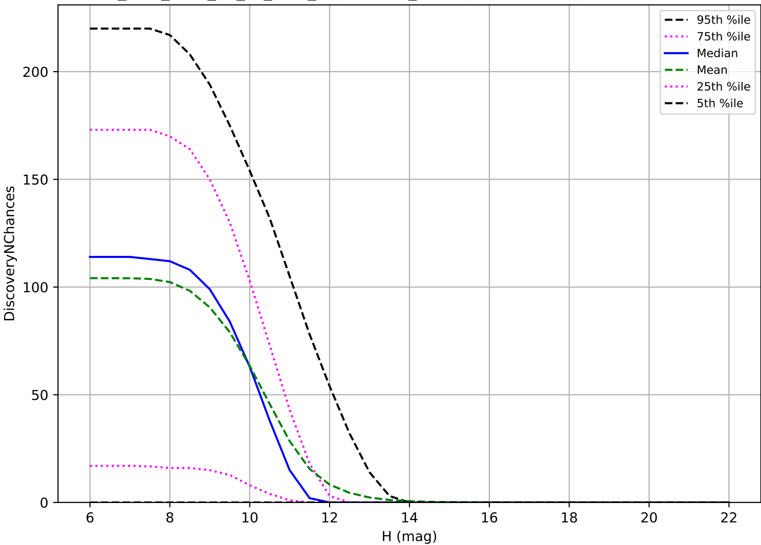
too_elab_r256_d3_gz_v3.4_10yrs: OCC_r20 3 pairs in 15 nights detection loss
